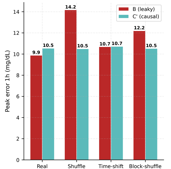
B (leaky) real vs controls shows large gap; C' (causal) real-vs-control gap is negligible
