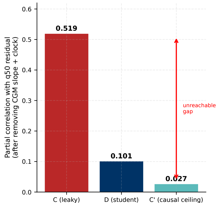
Leaky teacher (C) has 0.519 partial corr; causal features collapse to ~0.027-0.101
