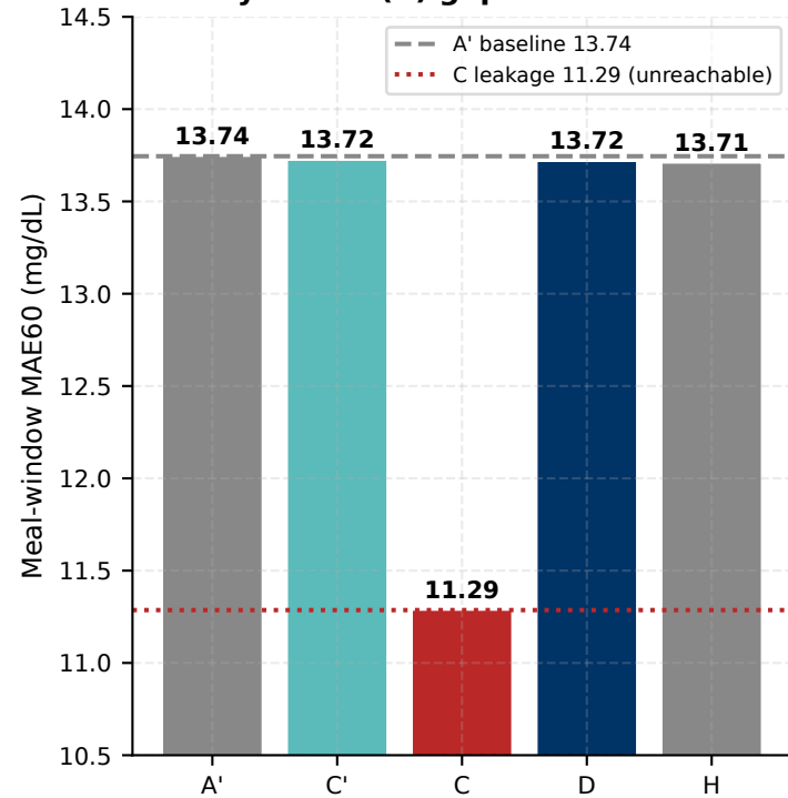
Causal ceiling (C') equals A'; leaky oracle (C) gap is unreachable
