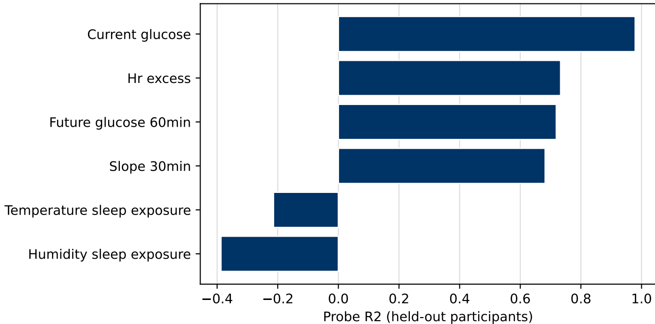
Regression targets, probe from h_t
