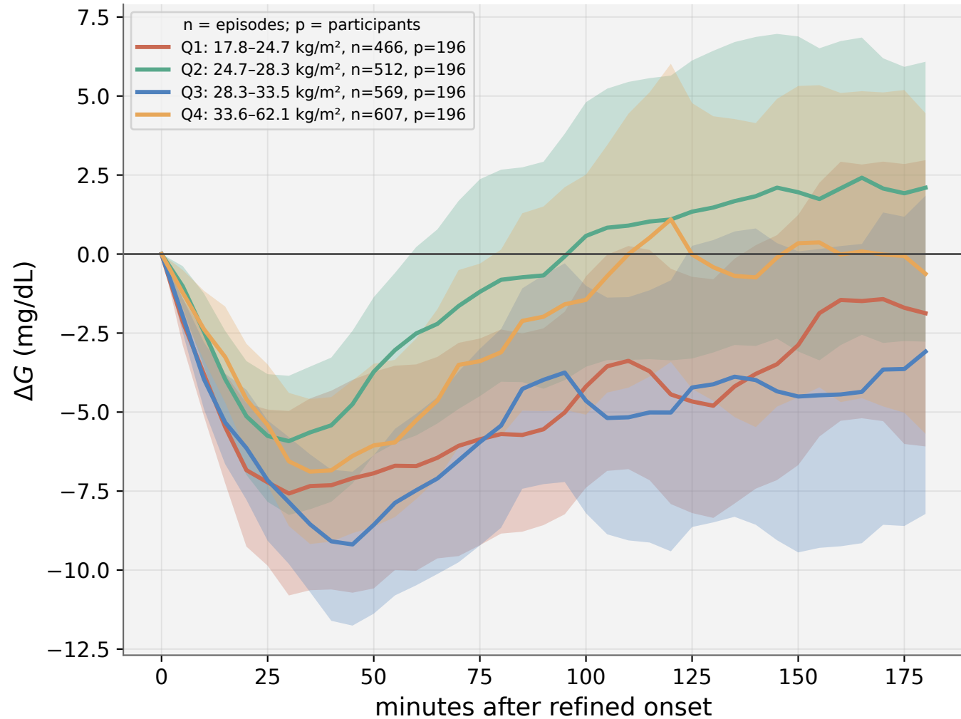
BMI quartile: response kernel
