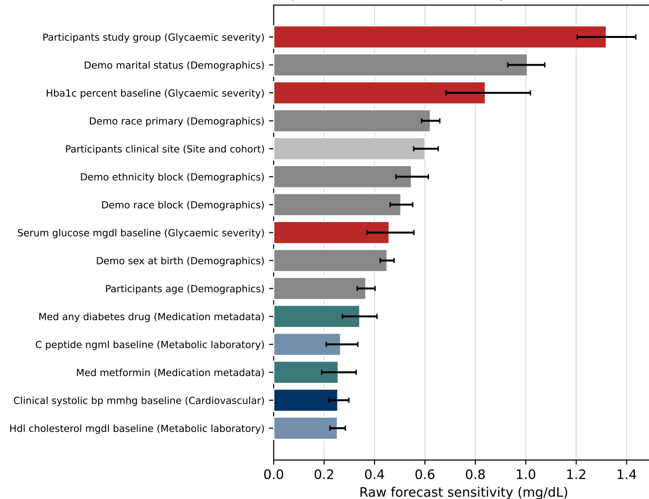
Top static features, sensitivity
