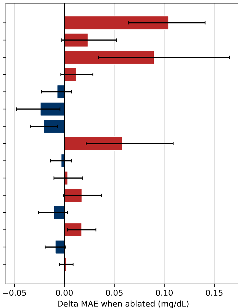
Top static features, predictive usefulness
