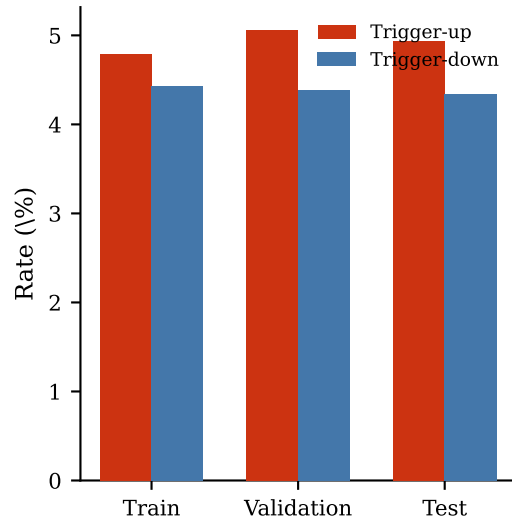
(c) Rates at locked \tau = 0.2
