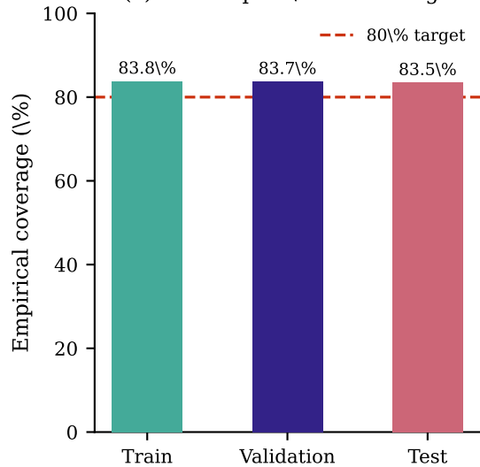
(a) One-step 80\% PI coverage
