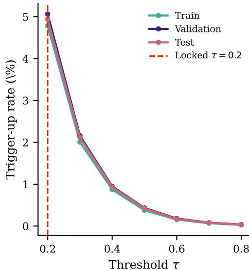
(b) Trigger rate vs. threshold
