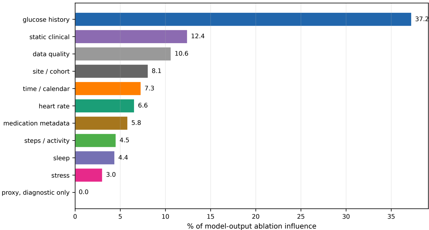
Global modality attribution for the frozen Study 2 model
