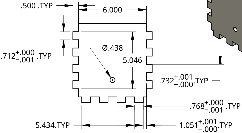
FRAME BACK 0.500 THICK
