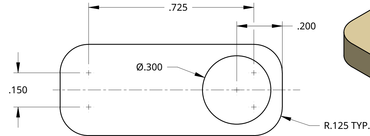
HALF TAB
