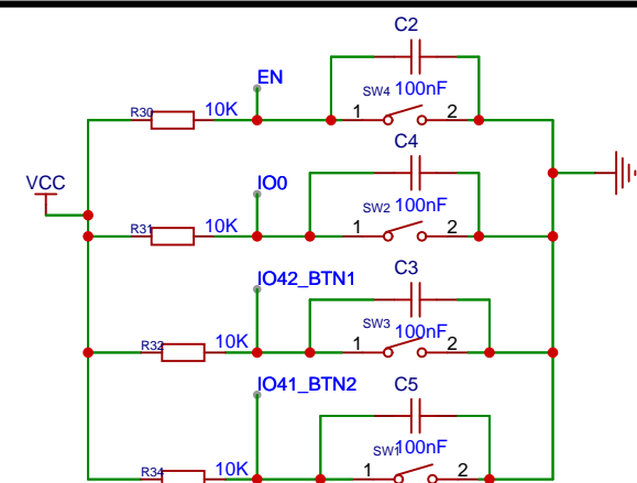
Button
