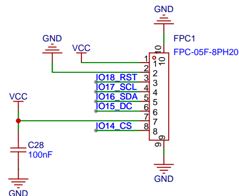
0.96inch Display
