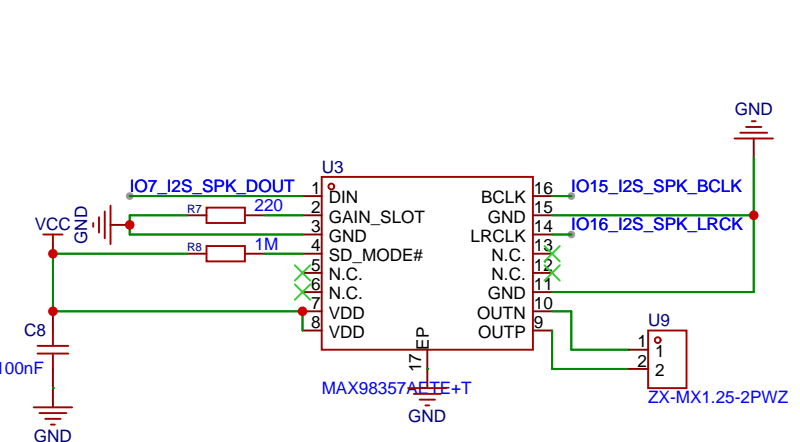
Speaker
