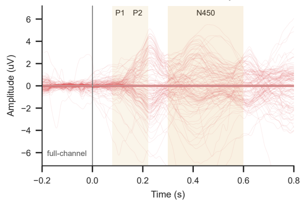
B CCD full-channel butterfly
