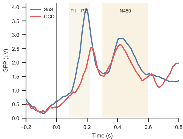
C Task overlay, global field power
