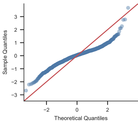
N450 residual QQ
