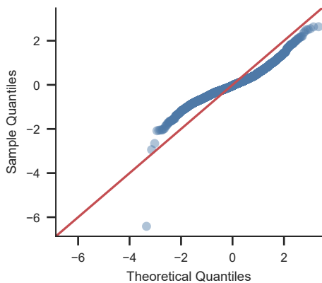
P2 residual QQ
