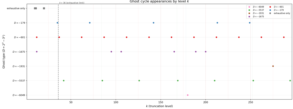
Figure 3: Ghost cycle appearances by level k . Each row represents a ghost type (identified by denominator D ). The vertical dashed line at k = 36 marks the boundary of exhaustive search; beyond it, ghost memberships are computed algebraically from Theorem 5. The periodic structure of case-(a) ghosts is clearly visible.
