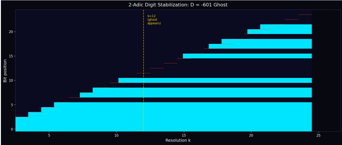
Figure 2: 2-adic digit stabilization for the D = -601 ghost ( L = 6 , V = 7 ). Each column shows the binary digits of n_1 = R \cdot D^{-1} \bmod 2^k . Digits stabilize from the least significant bit upward: once bit position b is determined at resolution k = b + 1 , it never changes. The dashed line marks k = 12 , where the ghost first materializes as a modular cycle.
