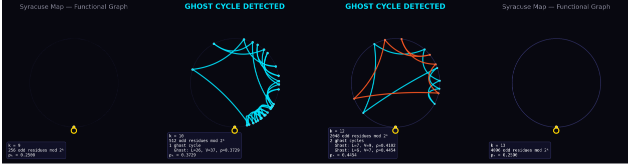
Figure 1: Chord diagrams of the Syracuse successor map at four resolutions. Odd residues mod 2^k are arranged around a circle; each arc connects a residue to its successor. At k = 9 and k = 13 (non-exceptional), only the fixed point \{1\} (gold) forms a cycle. At k = 10 , a 26-node ghost cycle appears (cyan). At k = 12 , two ghost cycles coexist (cyan: L = 7 , orange: L = 6 ).
