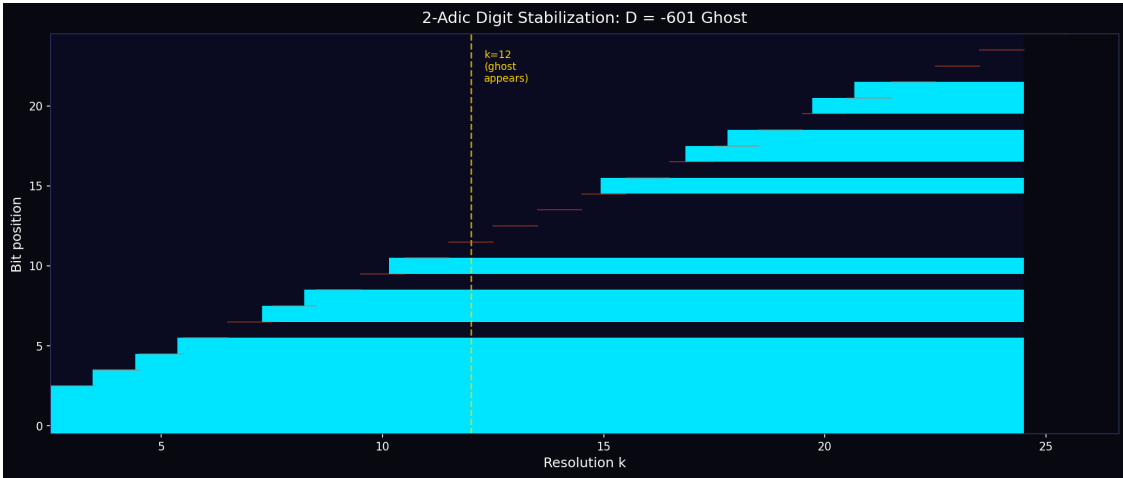
Figure 2: 2-adic digit stabilization for the D = -601 ghost ( L = 6 , V = 7 ). Each column shows the binary digits of n_1 = R \cdot D^{-1} \mod 2^k . Digits stabilize from the least significant bit upward: once bit position b is determined at resolution k = b + 1 , it never changes. The dashed line marks k = 12 , where the ghost first materializes as a modular cycle.
