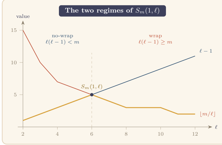
Figure 10. The single-class value S_m(1, \ell) = \min(\ell - 1, \lfloor m/\ell \rfloor) for m = 30 (Theorem 0.17). The rising line \ell - 1 (teal) governs the no-wrap regime; the falling curve \lfloor m/\ell \rfloor (terracotta) governs the wrap regime. The value S_m(1, \ell) (mustard) is the lower of the two: it climbs along \ell - 1 , peaks where the curves cross, here at \ell = 6 , exactly where \ell(\ell - 1) = m (dashed), then descends along \lfloor m/\ell \rfloor .
