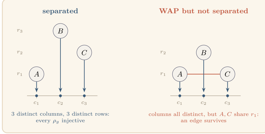
Figure 12. Separation versus whole-axis projection-injectivity (Definition 0.21). Left: a separated fiber: the three atoms occupy three distinct columns and three distinct rows, so \rho_{g1} and \rho_{g2} are both injective and, by the Coordinate-Union Edge Rule, G_{\text{atom}}[X_P] has no edges. The singleton coordinate-cliques along either axis are a minimum cover and the whole fiber is a maximum packing, so the residual-cover number is exact (Theorem 0.22). Right: a fiber that is WAP via the column axis but not separated: the columns are all distinct, yet A and C share the row residue r_1 , so the edge A-C survives and the fiber is not a packing. One injective axis therefore does not certify the cover number; here the cover may use the row clique \{A, C\} and beat the column count. Non-separated fibers are where the cover/packing deficit can appear (Section ).
