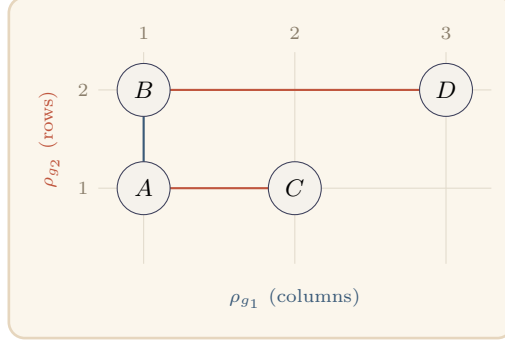
Figure 11. The Coordinate-Union Edge Rule (Theorem 0.19) for a two-axis fiber. Each atom is placed by its coordinates (\rho_{g_1}, \rho_{g_2}) , and two atoms are adjacent exactly when they share a column (same \rho_{g_1} , teal) or a row (same \rho_{g_2} , terracotta), “rook adjacency.” Here A, B share column 1, A, C share row 1, and B, D share row 2; the other three pairs differ in both coordinates and are non-adjacent. A fiber is whole-axis projection-injective (WAP) exactly when its atoms occupy distinct lines along one axis, e.g. distinct columns, so that axis alone separates every atom.
