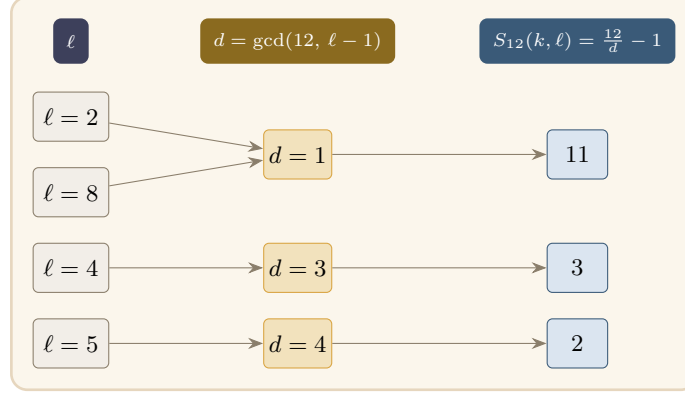
Figure 3. What the closed form says (Theorem 0.2, in the regime k \geq n - 1 ). The value S_m(k, \ell) = m / \gcd(m, \ell - 1) - 1 depends on \ell only through d = \gcd(m, \ell - 1) : the pair (m, \ell) collapses to the single quantity n = m/d , and the longest colorable list is n - 1 , one short of the self-defeating value n . With m = 12 fixed, \ell = 2 and \ell = 8 share d = 1 (both \ell - 1 coprime to 12), so both give S_{12} = 11 ; \ell = 4, 5 give 3, 2.
