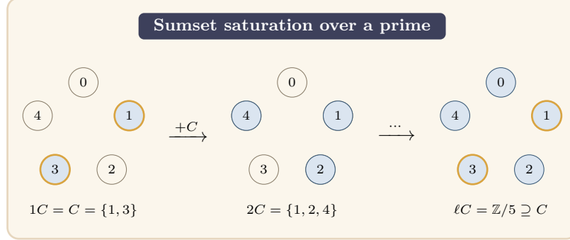
Figure 8. Saturation over a prime modulus (Theorem 0.13), for C = \{1, 3\} \subseteq \mathbb{Z}/5 . Since \langle C - C \rangle = \mathbb{Z}/5 (a prime has no proper nontrivial subgroup), the \ell -fold sumsets grow 1C \subset 2C \subset \dots and fill the whole group after at most |H| - 1 = 4 steps. The filled set \ell C = \mathbb{Z}/5 then contains C itself (mustard ring), so some \ell -sum of elements of C equals an element of C , and the class is not \ell -sum-free. The same collapse hits every class of size \geq 2 over a prime, so only singletons survive and k_0(p, \ell) = p - 1 (Corollary 0.15).
