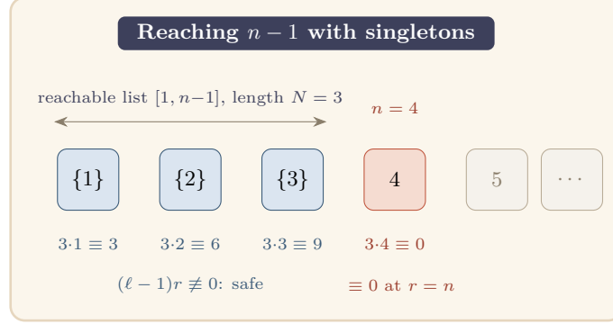
Figure 7. The matching lower bound for m = 12 , \ell = 4 (so n = 4 ). Each of 1, 2, \dots, n - 1 goes in its own singleton class; by Lemma 0.5 the class \{r\} is \ell -sum-free exactly when (\ell - 1)r \not\equiv 0 \pmod{m} , that is when n \nmid r , which holds for every r < n . The construction therefore colors all of [1, n - 1] and reaches N = n - 1 = 3 . It stops there because the list must be an initial segment [1, N] , and the next value n = 4 is the self-defeating singleton (\ell - 1)n \equiv 0 , which caps the list (compare Figure 5).
