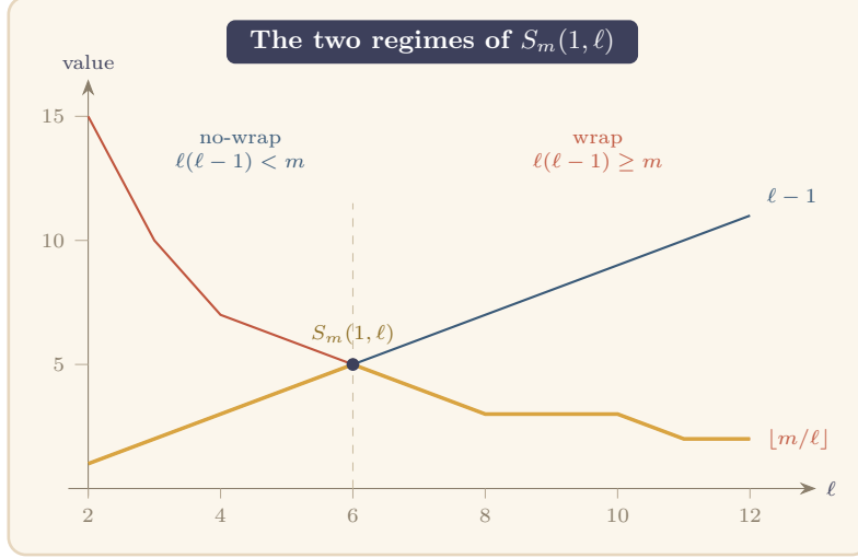
Figure 10. The single-class value S_m(1, \ell) = \min(\ell - 1, \lfloor m/\ell \rfloor) for m = 30 (Theorem 0.17). The rising line \ell - 1 (teal) governs the no-wrap regime; the falling curve \lfloor m/\ell \rfloor (terracotta) governs the wrap regime. The value S_m(1, \ell) (mustard) is the lower of the two: it climbs along \ell - 1 , peaks where the curves cross, here at \ell = 6 , exactly where \ell(\ell - 1) = m (dashed), then descends along \lfloor m/\ell \rfloor .
