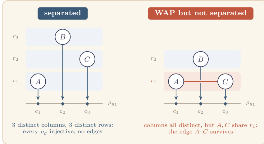
Figure 12. Separation versus whole-axis projection-injectivity (Definition 0.21). The shaded bands are the residue classes along the row axis g_2 : each band is one coordinate-clique. Left : a separated fiber: the three atoms occupy three distinct columns and three distinct rows, so \rho_{g_1} and \rho_{g_2} are both injective and, by the Coordinate-Union Edge Rule, G_{\text{atom}}[X_P] has no edges. The singleton coordinate-cliques along either axis are a minimum cover and the whole fiber is a maximum packing, so the residual-cover number is exact (Theorem 0.22). Right : a fiber that is WAP via the column axis but not separated: the columns are all distinct, yet A and C share the row residue r_1 , so the edge A-C survives and the fiber is not a packing. One injective axis therefore does not certify the cover number; here the cover may use the row clique \{A, C\} and beat the column count. Non-separated fibers are where the cover/packing deficit can appear (Section ).
