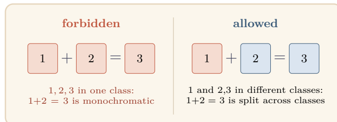
Figure 1. The Schur coloring game: a coloring of 1, \dots, N is valid when no class contains a solution of x+y=z , here 1+2=3 . The valid 2-coloring \{1, 4\}, \{2, 3\} of \{1, \dots, 4\} gives S(2) = 4 . This paper forbids instead the longer congruence x_1 + \dots + x_\ell \equiv y \pmod{m} .
