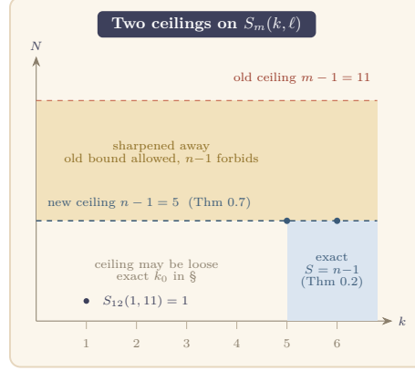
Figure 6. The two ceilings for m = 12 , \ell = 11 (so d = 2 , n = 6 ). The old universal bound S_m(k, \ell) \leq m - 1 = 11 (Lemma 0.4) is sharpened to S_m(k, \ell) \leq n - 1 = 5 (Theorem 0.7); the mustard band between the two dashed lines is forbidden by the new bound but was permitted by the old one. The bound is attained with equality, S = n - 1 , once k \geq n - 1 (teal column, Theorem 0.2); for fewer classes it can be strictly loose, e.g. S_{12}(1, 11) = 1 , and the exact threshold k_0 is the subject of §.
