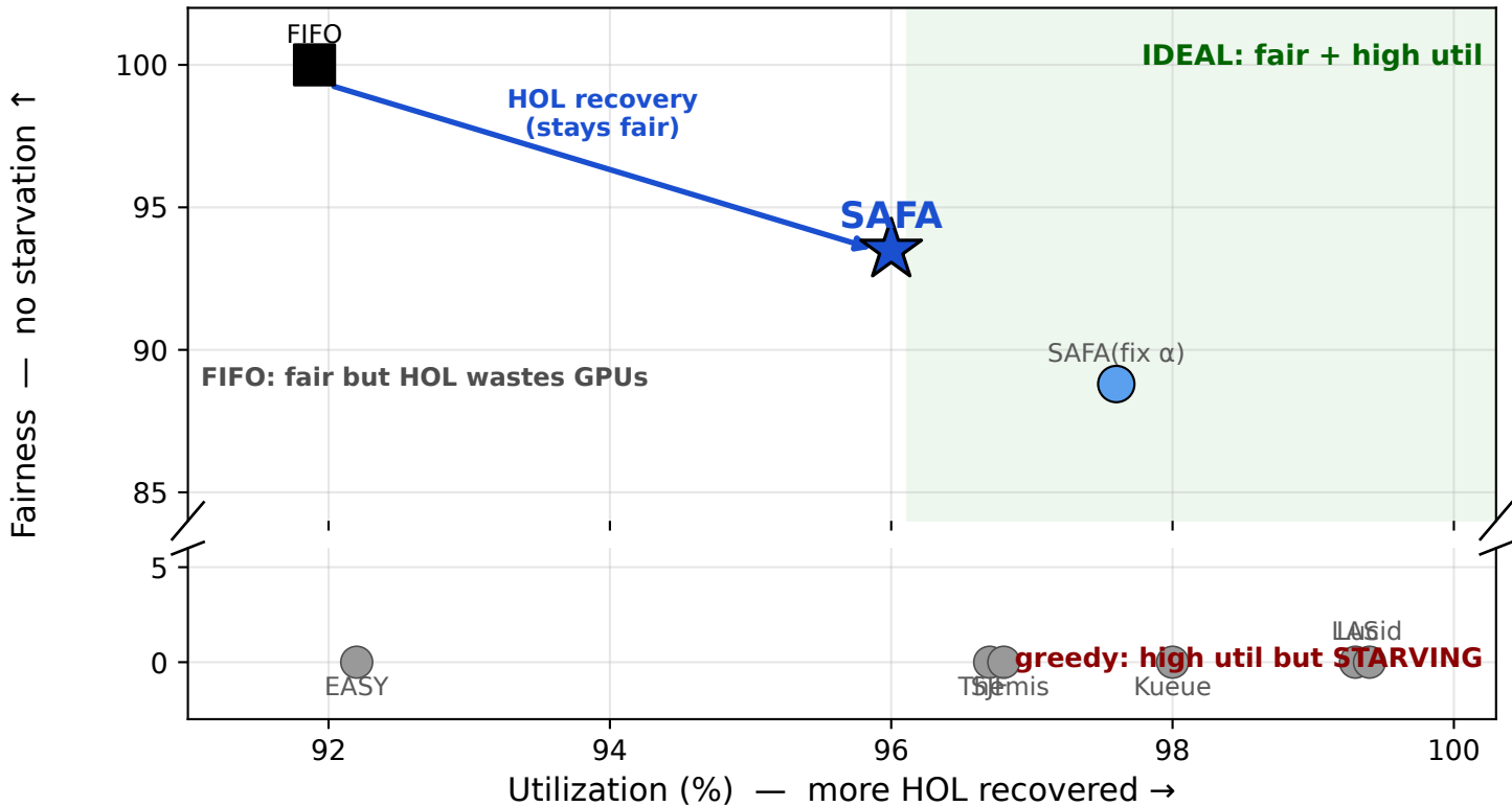
Utilization × Fairness (256 single, overload) — only SAFA is fair AND high-util
