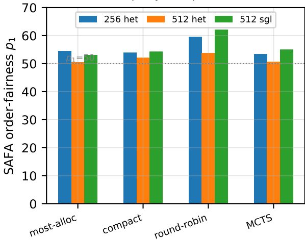
SAFA p_1 by core placement
