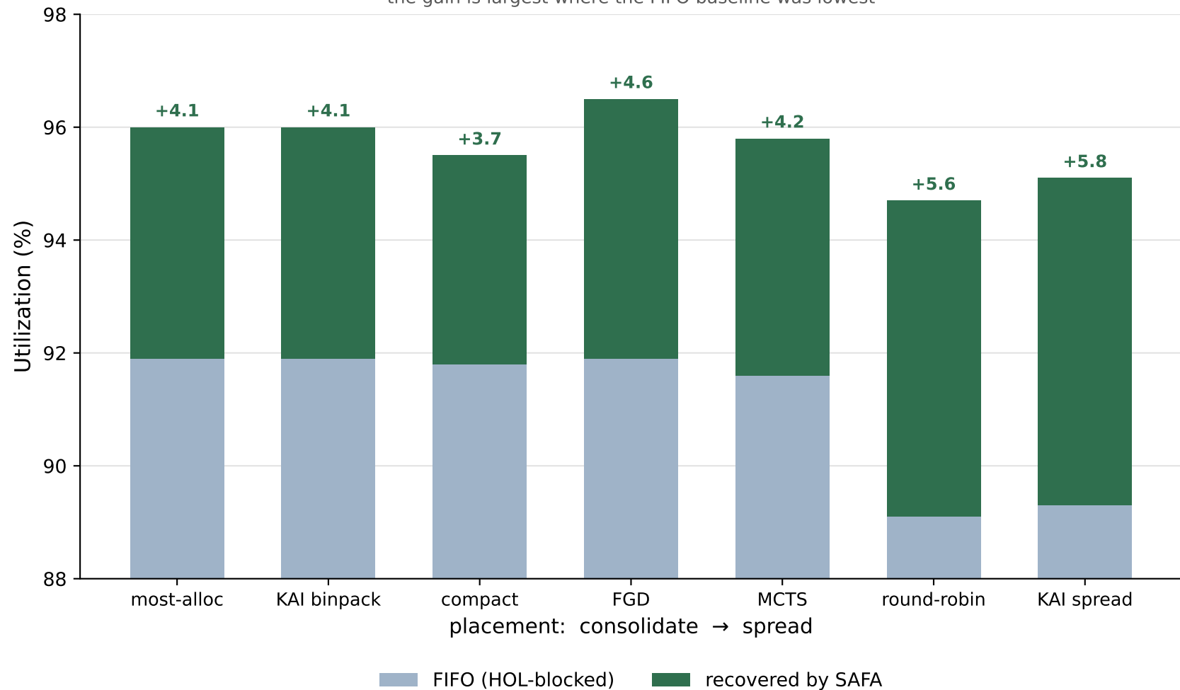
SAFA raises utilization under every placement (256 GPUs, single; SAFA Fairness 91.8-93.7) the gain is largest where the FIFO baseline was lowest
