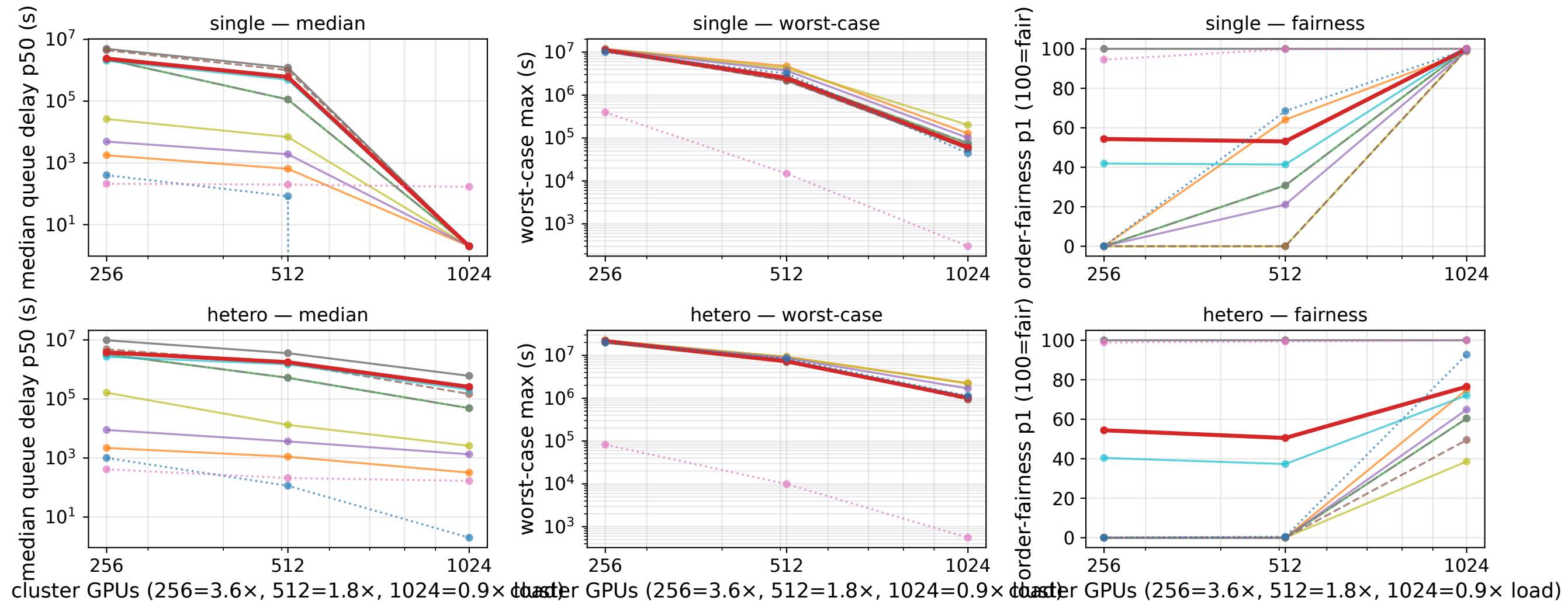
Load dependence, all 11 policies (Philly 111k): single (top) vs heterogeneous (bottom)
