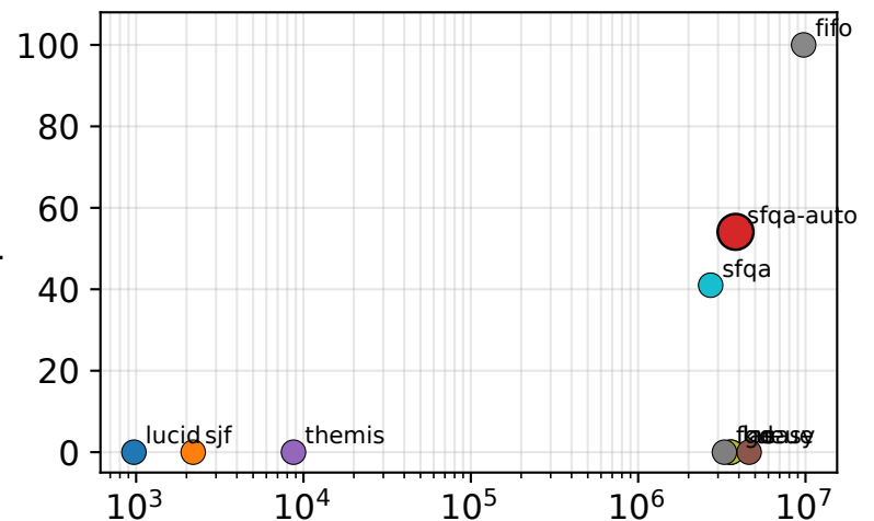
256 GPU hetero (3.6×)
