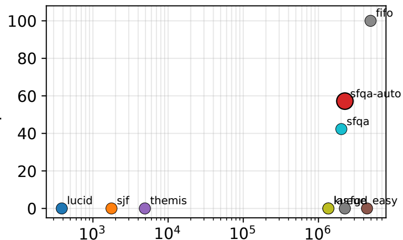
256 GPU single (3.6×)
