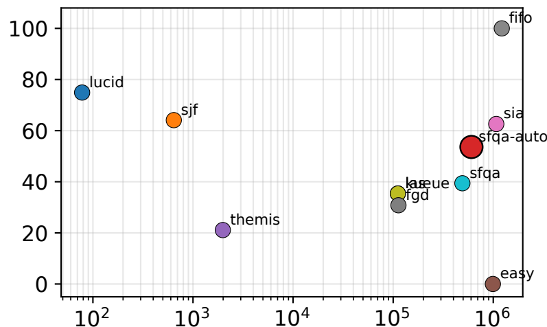
512 GPU single (1.8×)
