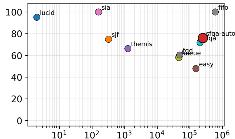
1024 GPU hetero (0.9×)
