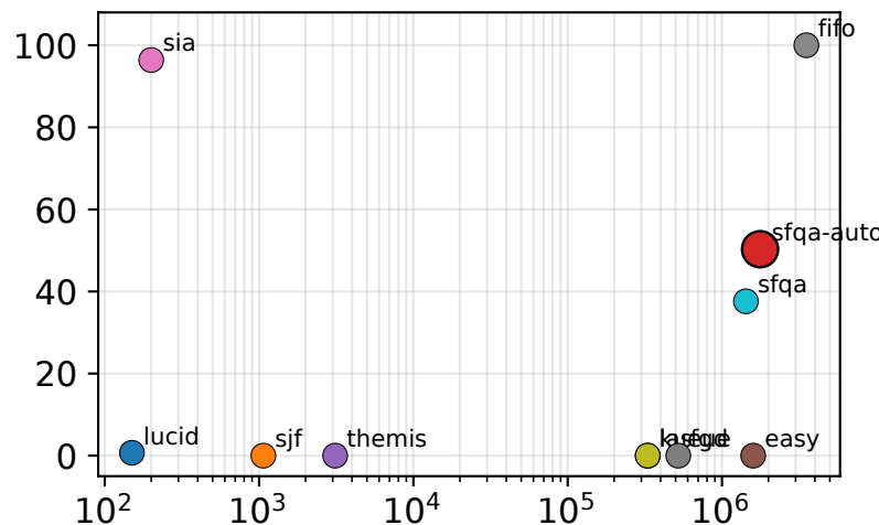
512 GPU hetero (1.8×)
