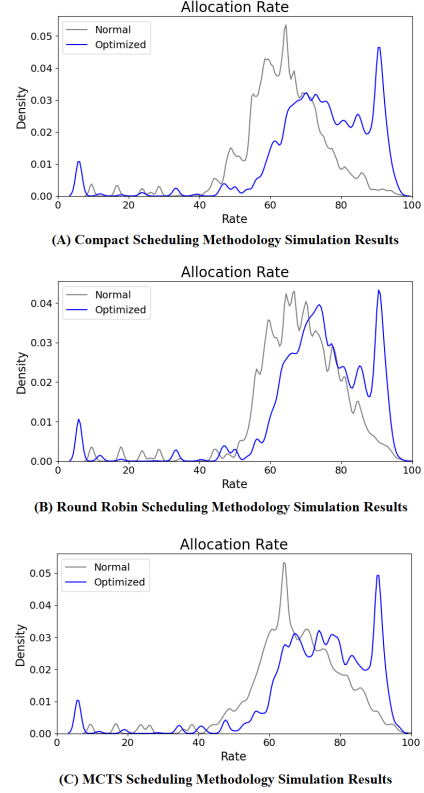
Fig. 11. Allocation rate comparison of various scheduling methodologies.
