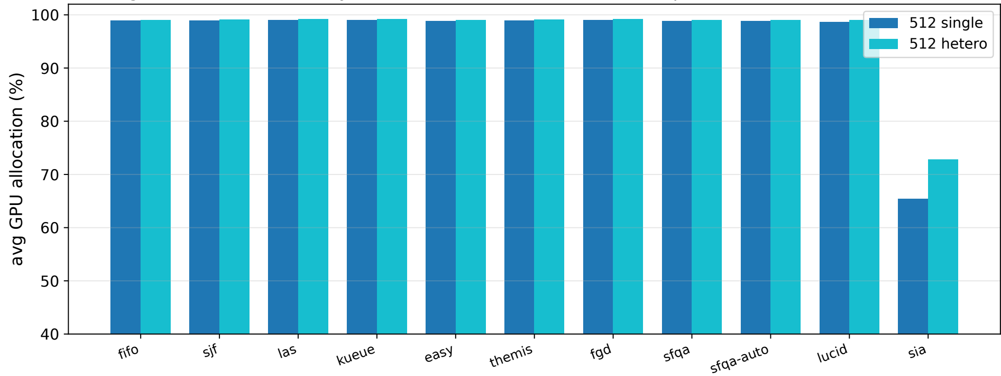
Average GPU allocation (Philly 111k, 512 GPU): all near 99% except Sia (elastic ILP leaves GPUs idle)
