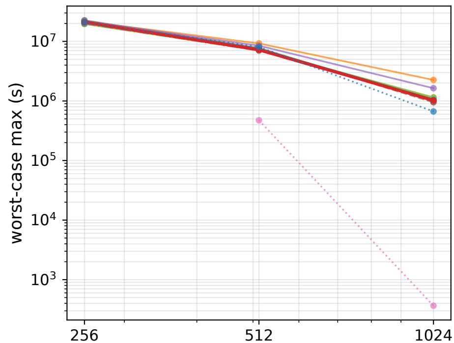
Load dependence on heterogeneous clusters (Philly 111k, all policies)
