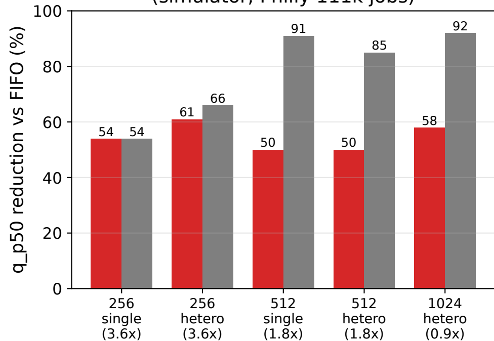
Both cut median vs FIFO (simulator, Philly 111k jobs)
