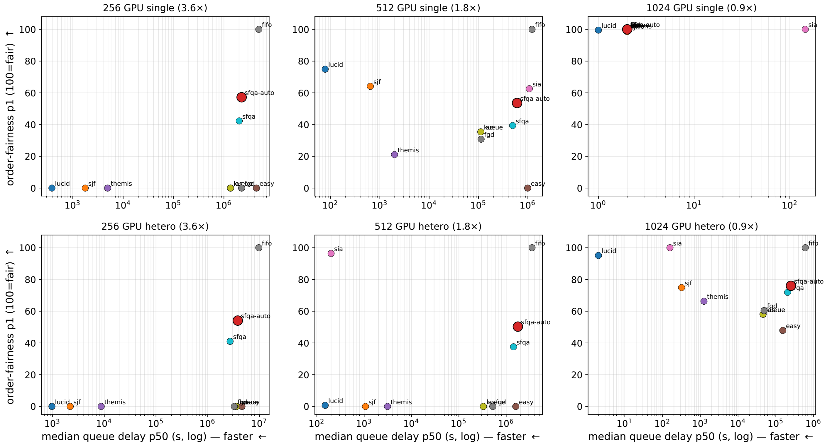
Queue-delay vs fairness trade-off, all 11 policies (Philly 111k): top-left = fast & fair (sfqa-auto's target region)
