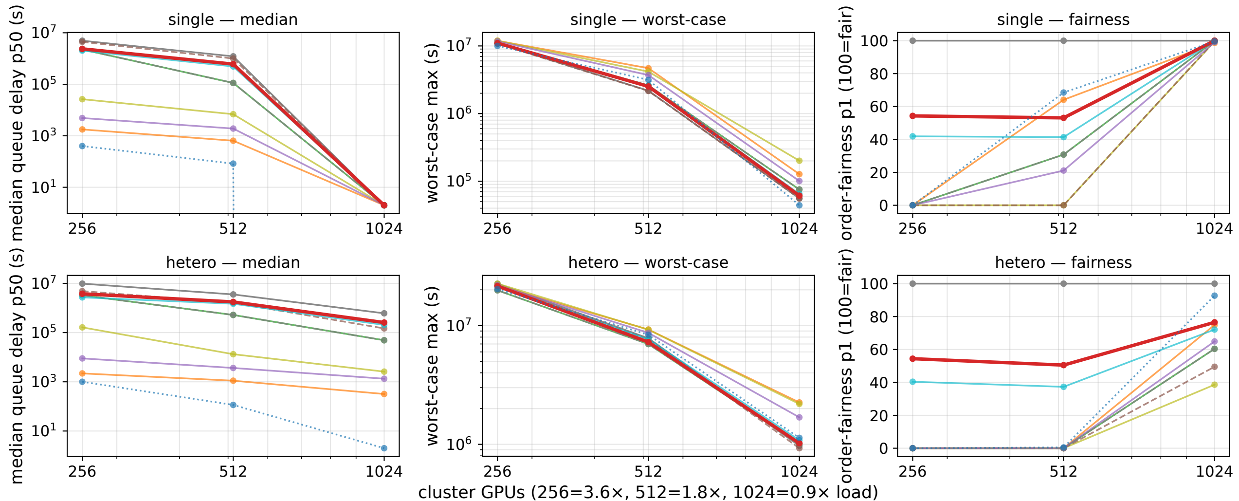
Load dependence, all 10 policies (Philly 111k): single (top) vs heterogeneous (bottom)
