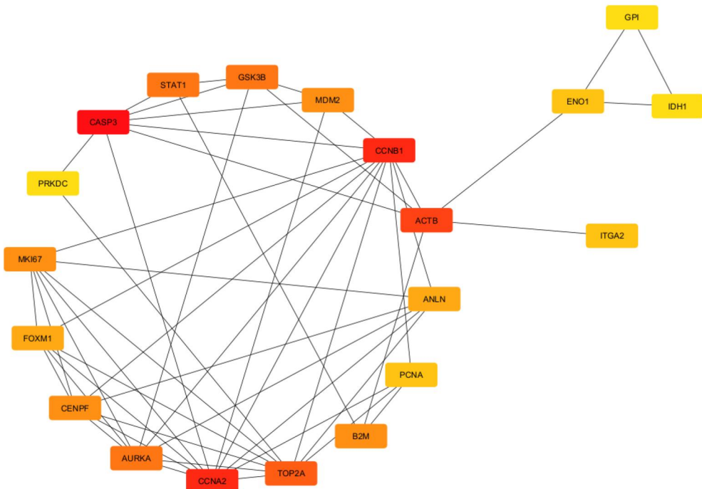
MCC-ranked network
