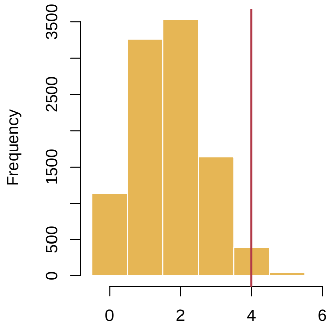
Robustness-label permutation
