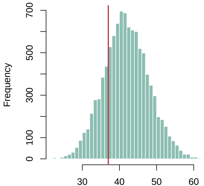
Gene-identity permutation
