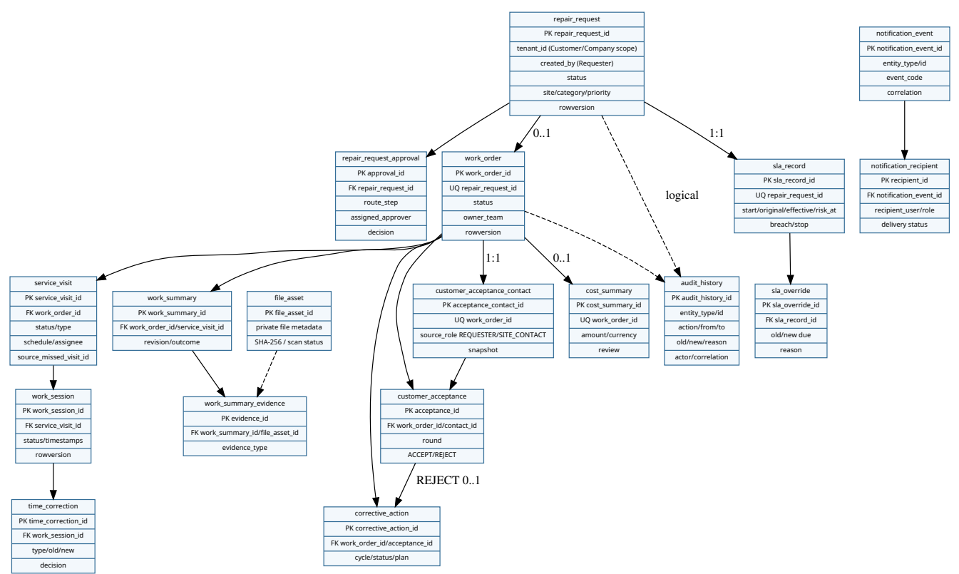
Figure 1 - Logical/physical entity baseline including NotificationRecipient and corrected acceptance contact semantics.
