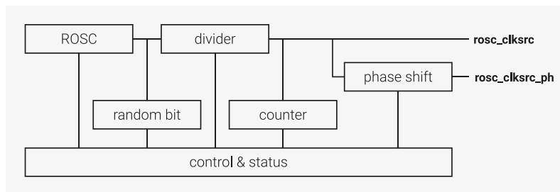
Figure 39. ROSC overview.
