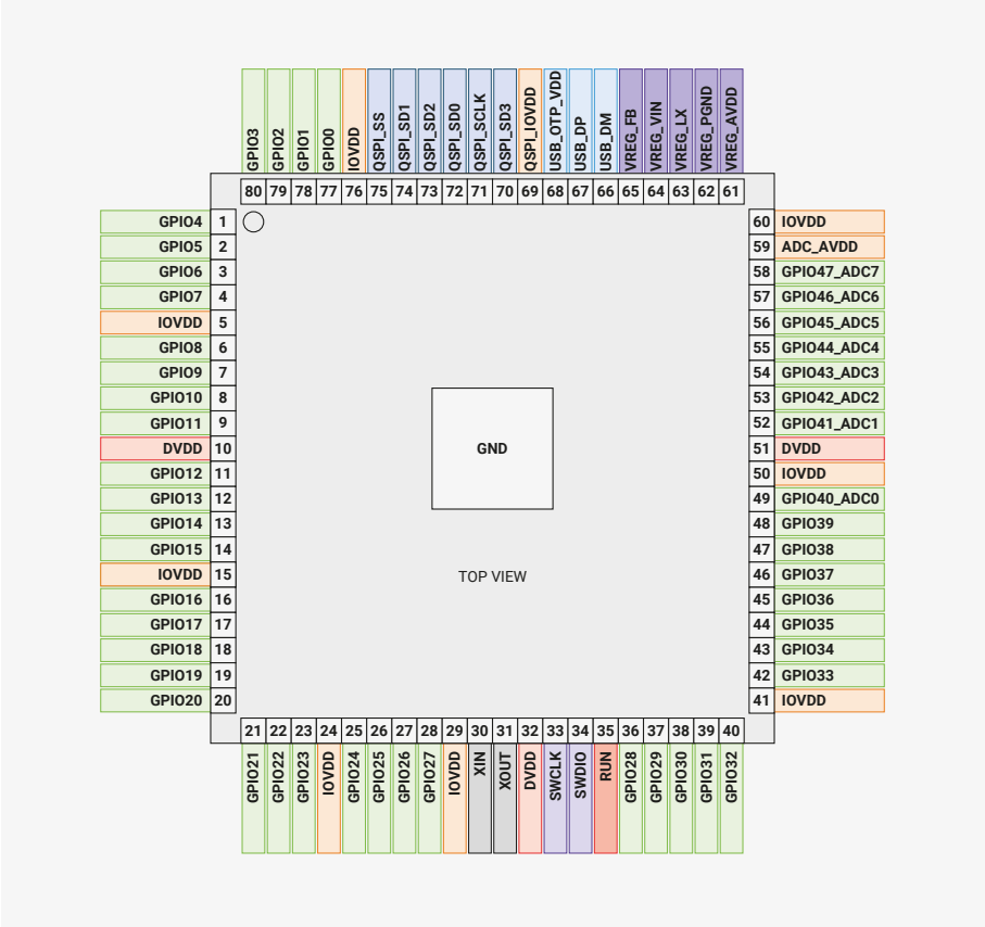
Figure 149. RP2350 Pinout for QFN-80 10×10mm
