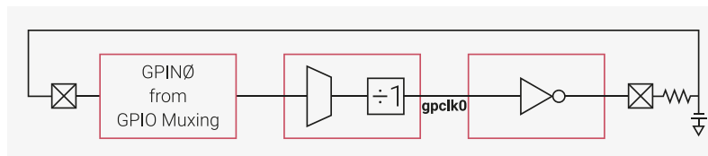
Figure 34. Simple relaxation oscillator example
