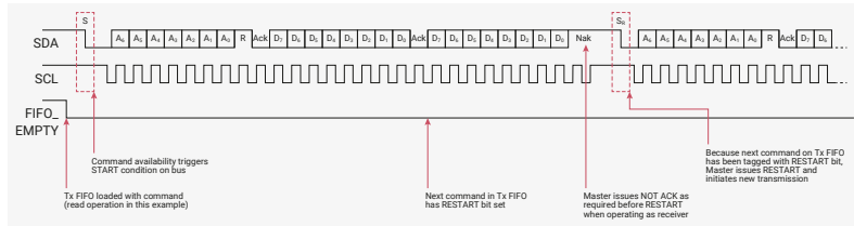
Figure 80. Master Receiver - Restart Bit of IC_DATA_CMD Is Set
