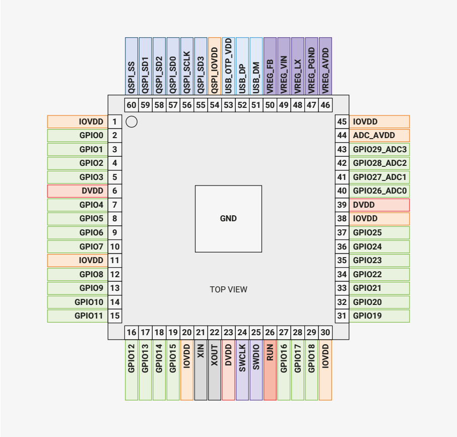
Figure 148. RP2350 Pinout for QFN-60 7×7mm
