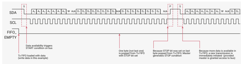
Figure 81. Master Transmitter - Stop Bit of IC_DATA_CMD Set/TX FIFO not empty
