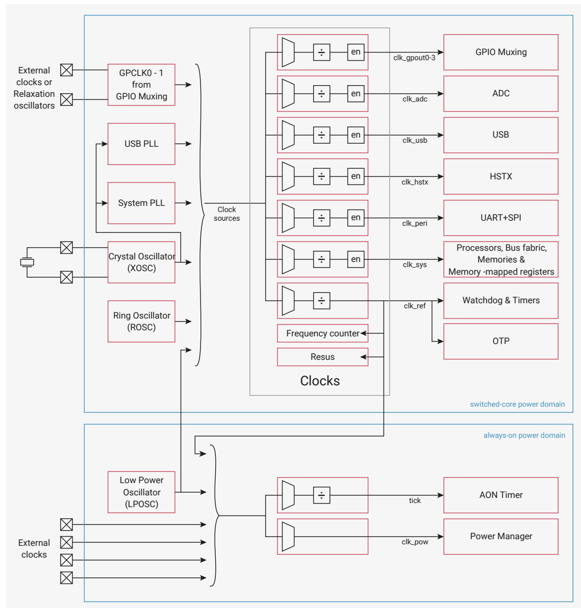
Figure 33. Clocks overview
