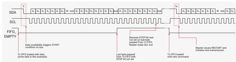
Figure 82. Master Transmitter - First Byte Loaded Into TX FIFO Allowed to Empty, Restart Bit Set
