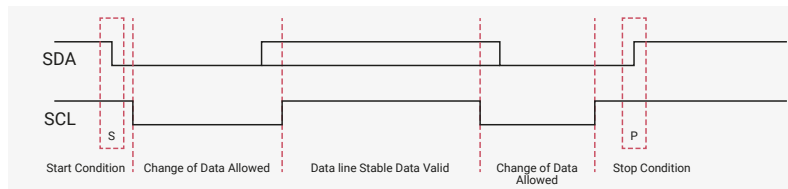
Figure 70. I2C START and STOP Condition
