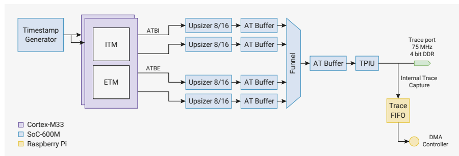
Figure 11. Trace Subsystem
