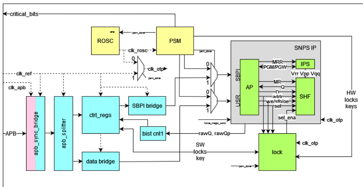
Figure 142. OTP architecture
