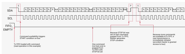
Figure 83. Master Receiver - Stop Bit of IC_DATA_CMD Set/TX FIFO Not Empty
