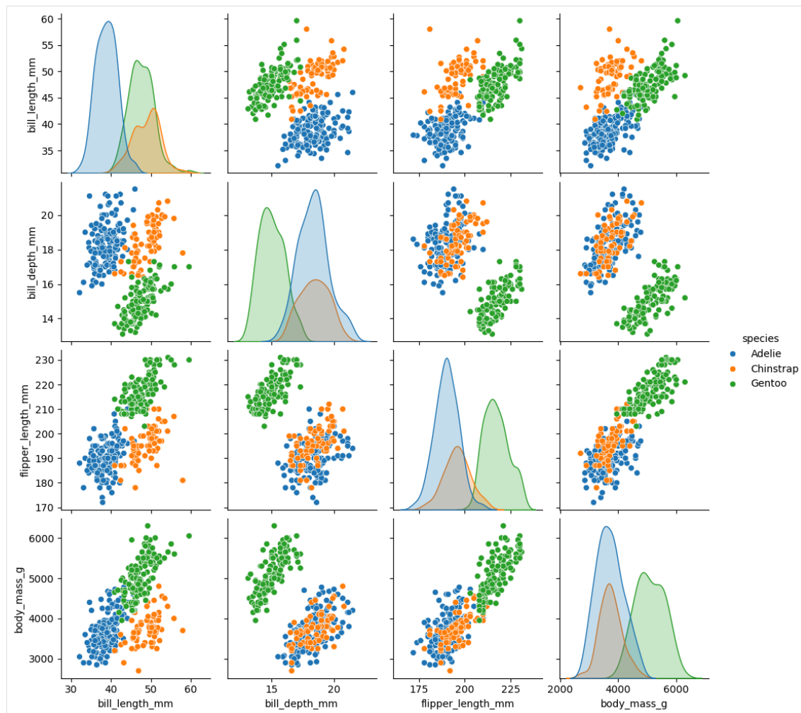
Scatter Plot – Joint Distribution of the flipper_length_mm and bill_depth_mm Continuous Variables
