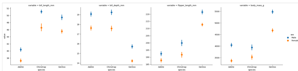
Point Plot – Mean and Confidence Interval of the flipper_length_mm Continuous Variable, Grouped by Each species Categorical Variable
