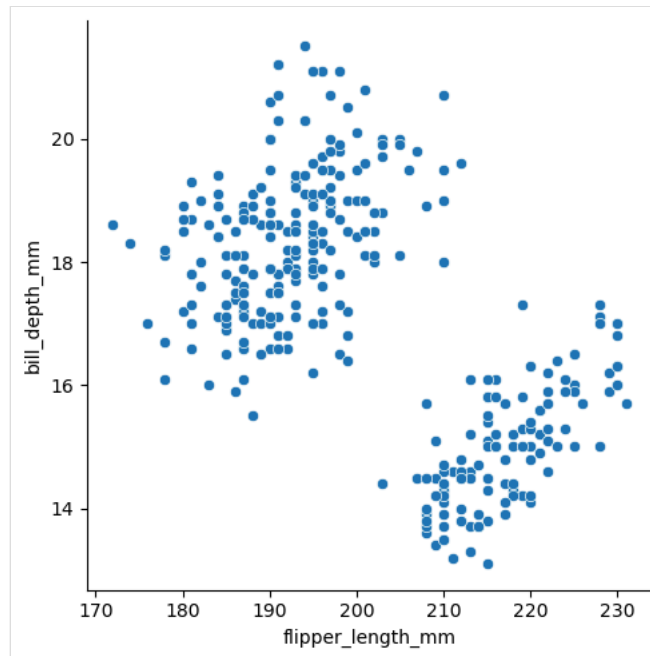
Scatter Plot – Joint Distribution of the bill_depth_mm and flipper_length_mm Continuous Variables
