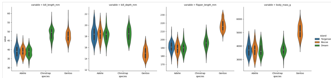
Violin Plot – Marginal Distribution Density of the body_mass_g Continuous Variable, Grouped by Each species Categorical Variable
