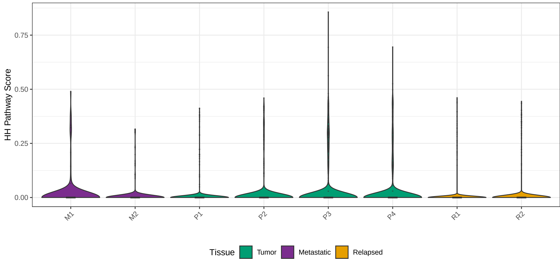
Hedgehog Pathway Score by Patient (Malignant Cells)
