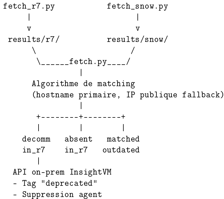
Figure 4: Pipeline RapidETNIC
