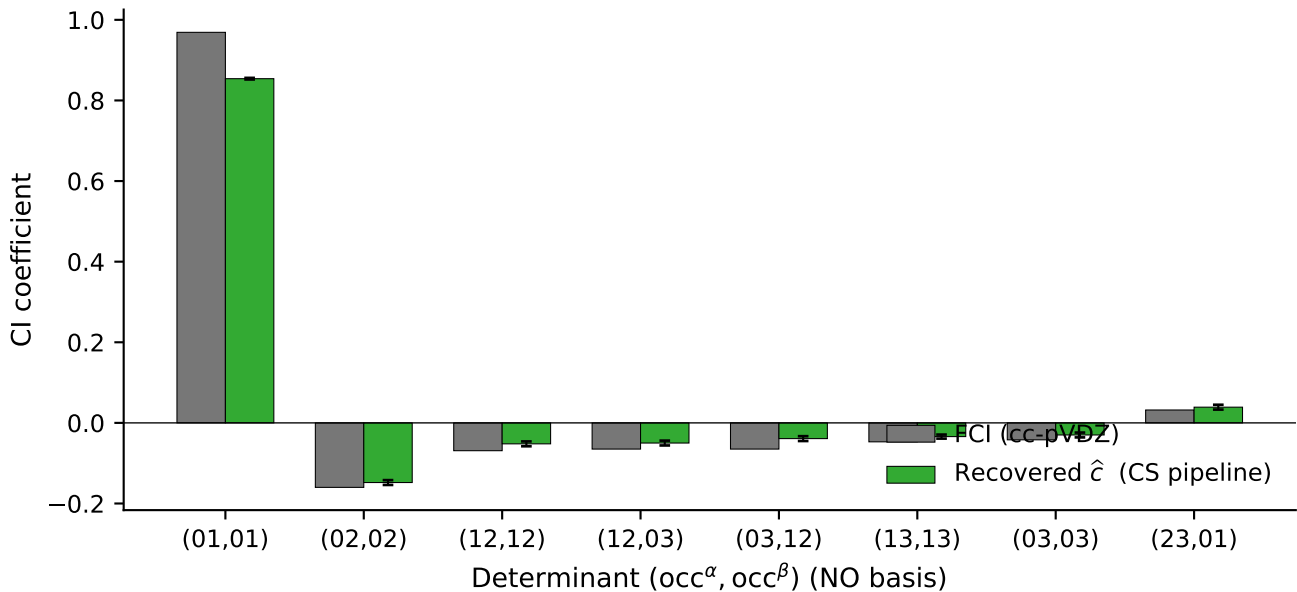
Linear H_4 / cc-pVDZ, R = 1.0 , AA: top-8 determinant recovery
