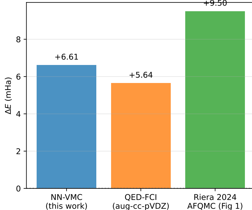
T2: Riera setting ( R = 1.4 , \omega = 0.3 Ha, \lambda = 0.1 )
