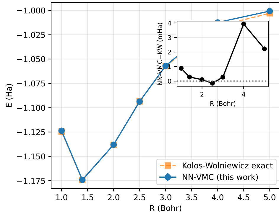
T1: Bare H 2 dissociation curve
