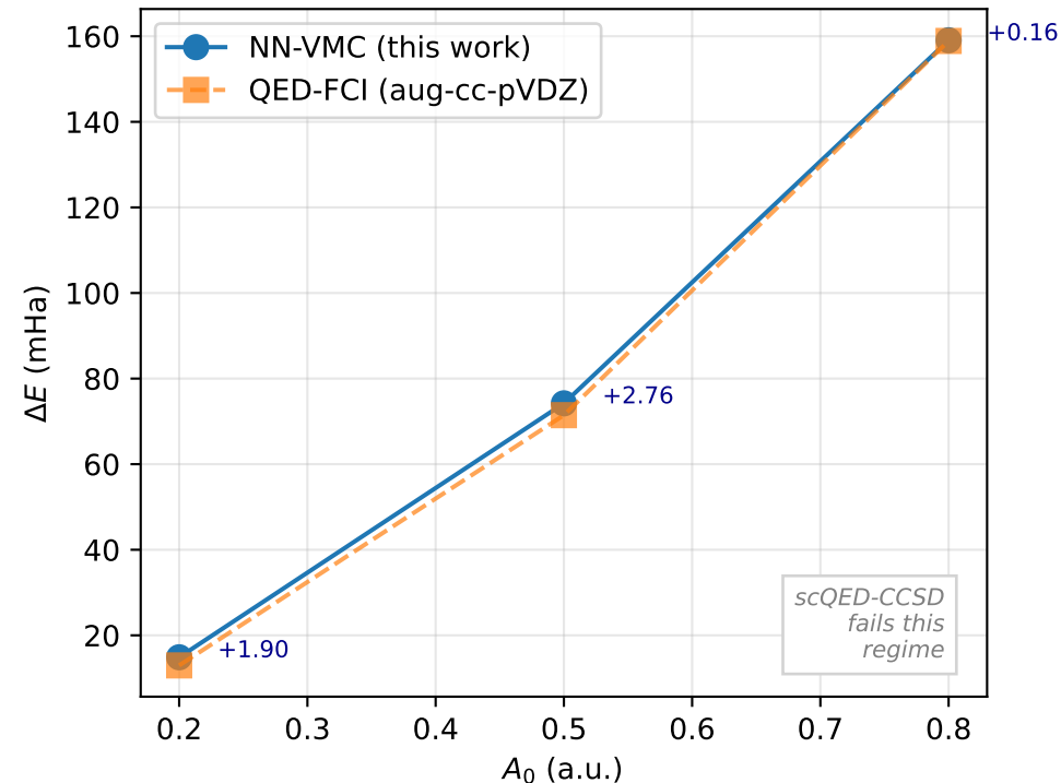
T3: Weight setting ( R = 2.8 , \omega_c = 5 eV)
