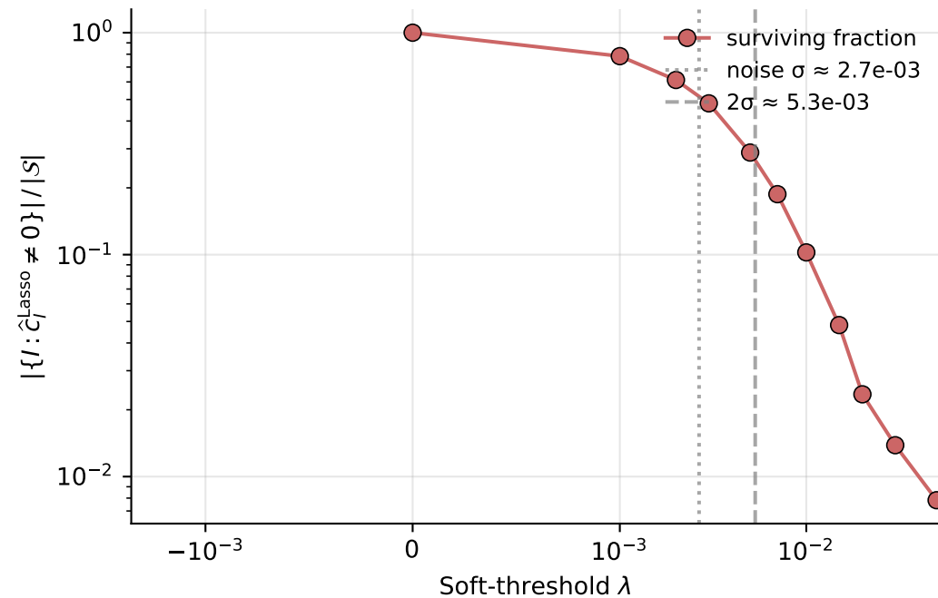
Lasso compression rate ( |S| = 1,661 )
