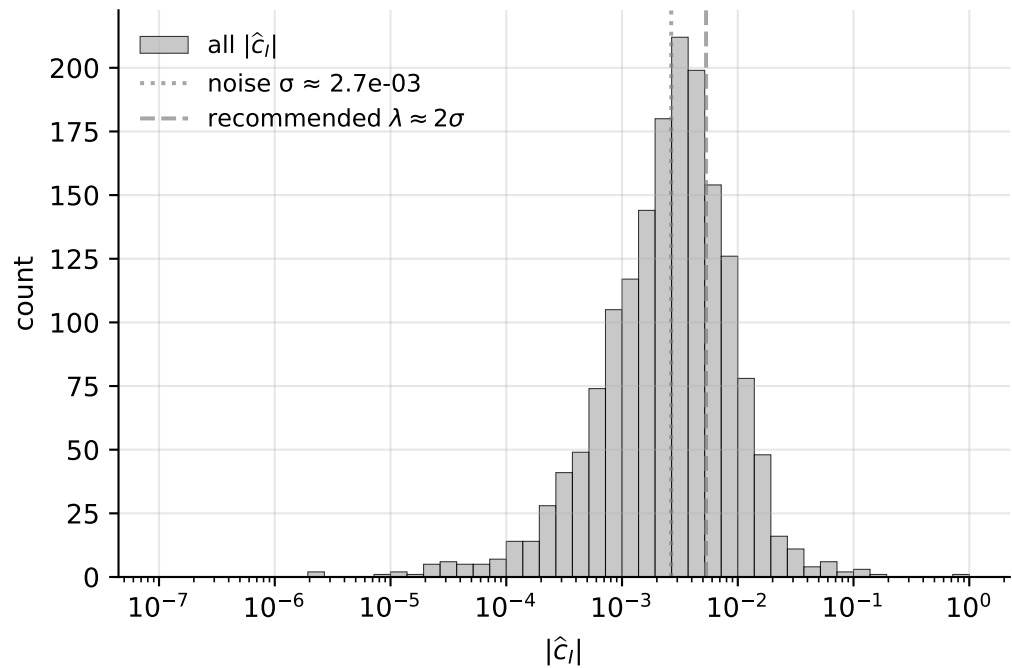
Distribution of |\hat{c}_l| — noise vs signal gap
