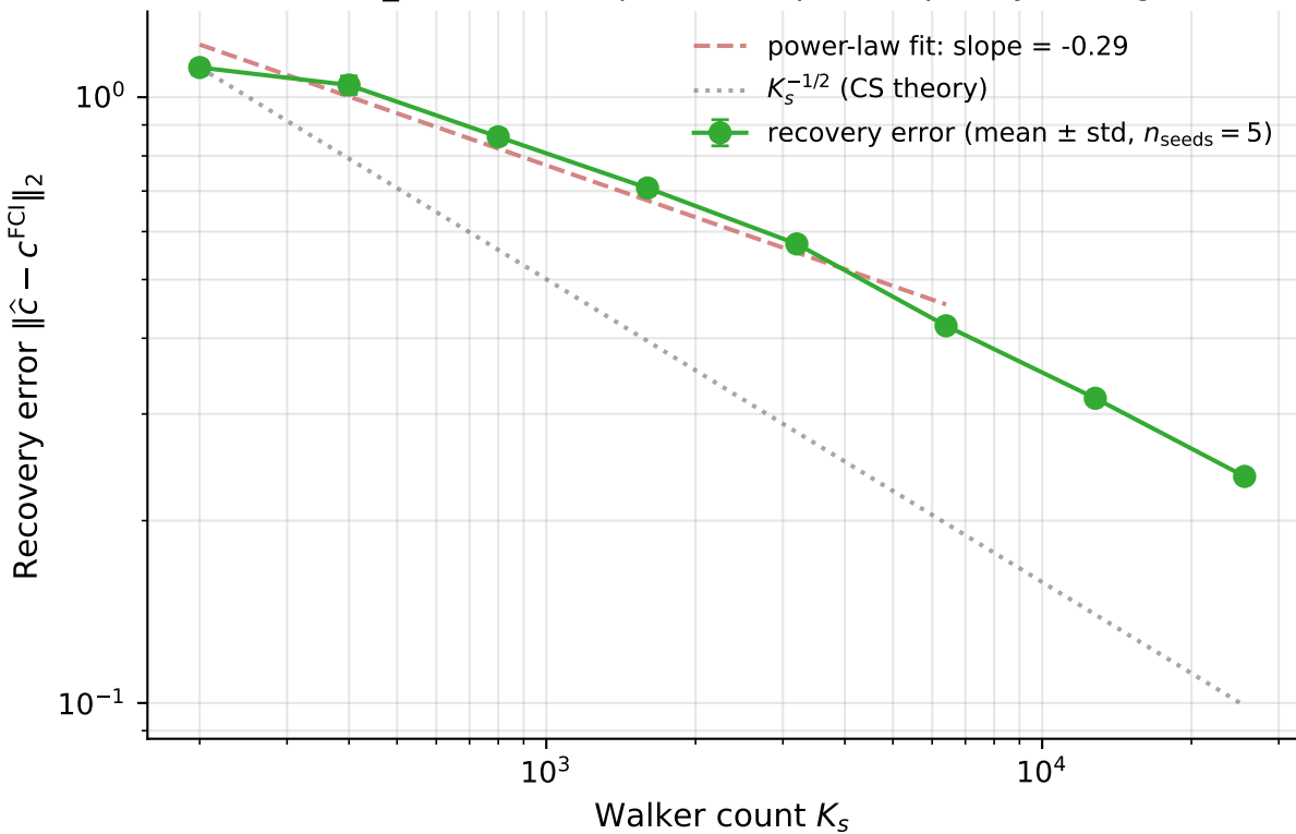
\text{H}_4 linear / cc-pVDZ: sample-complexity scaling
