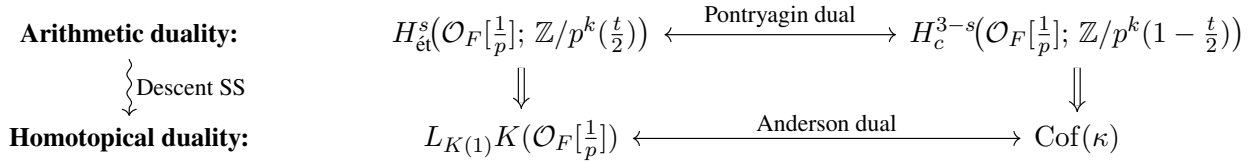
Figure 2: Arithmetic and homotopical dualities in parallel, linked by the descent spectral sequence.
