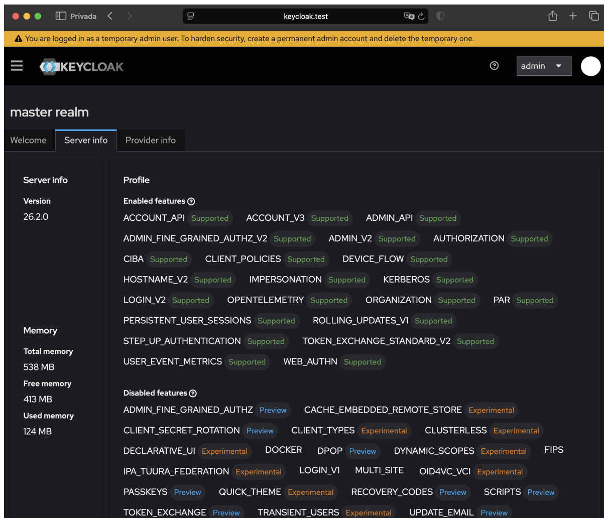
Figure 6. User interface of Keycloak
