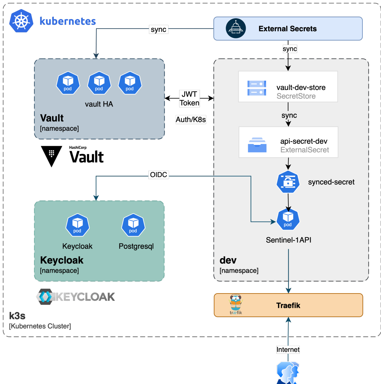
Figure 1. Seminar Architecture
