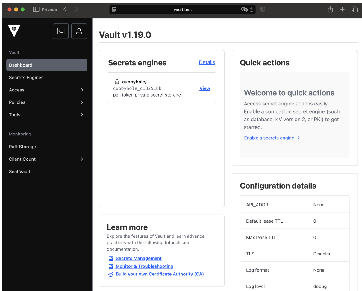
Figure 2. Vault dashboard
