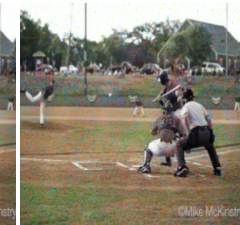
T=1.5
