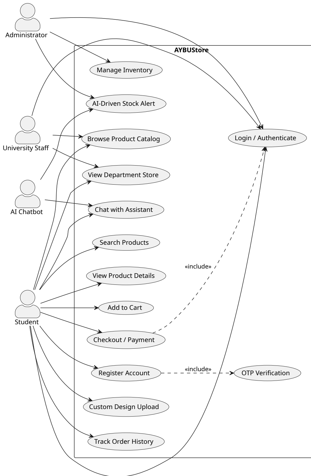
Figure 1: AYBUStore Use Case Diagram (Vector)
