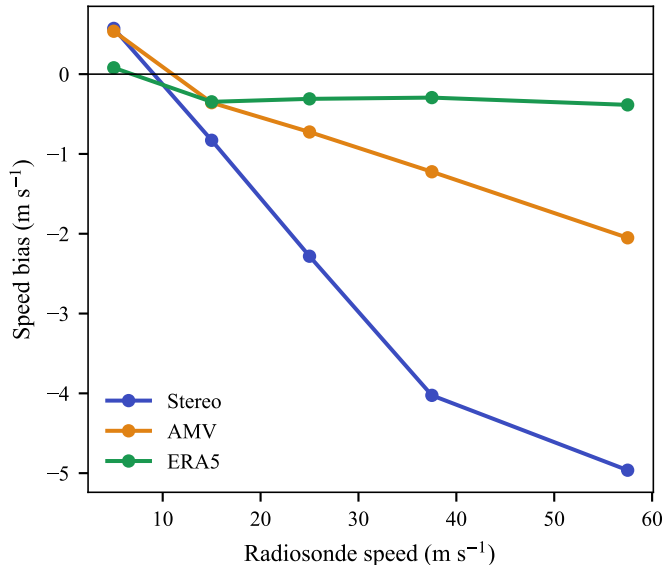
(b) Speed bias vs wind speed
