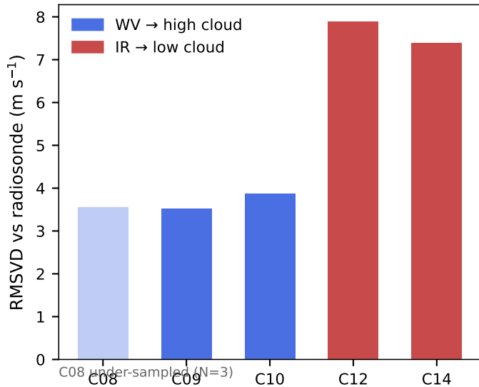
(b) Per-band RMSVD
