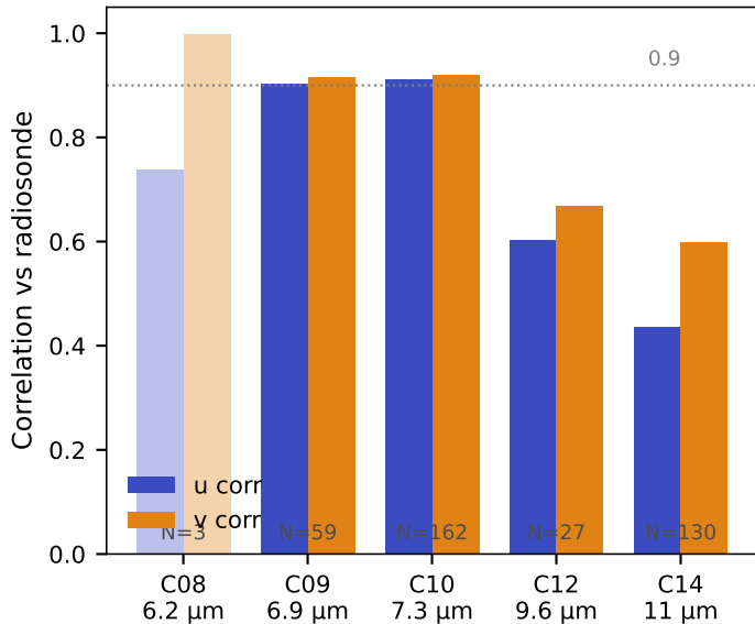
(a) Per-band wind correlation
