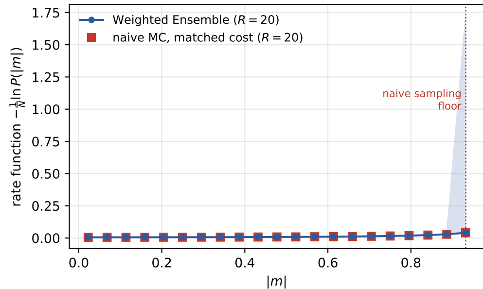
(a) WE reaches beyond naive's hard support floor (shaded: \pm 1 s.d. over 20 replicas)
