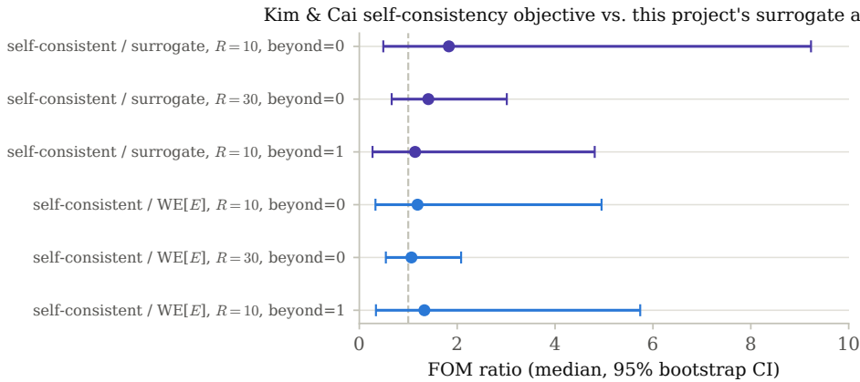
Figure 3: All six FOM-ratio comparisons from Tables 7 and 8 as a forest plot. Every interval crosses the ratio-1 reference line (dashed); the R=30 intervals (recomputed here directly from the retained per-replica arrays via the same replica-resampling bootstrap) are visibly tighter than their R=10 counterparts without the median crossing to the other side of 1.
