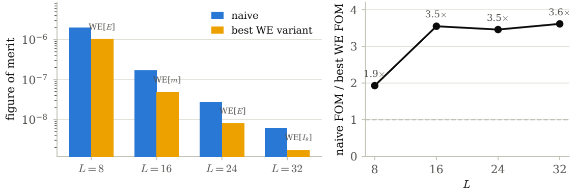
Figure 4: Table 11 as a figure. Left: naive vs. best WE-variant FOM by L , log scale, labeled with which variant won. Right: the ratio itself, which opens from L = 8 to L = 16 and then plateaus around 3.5×
