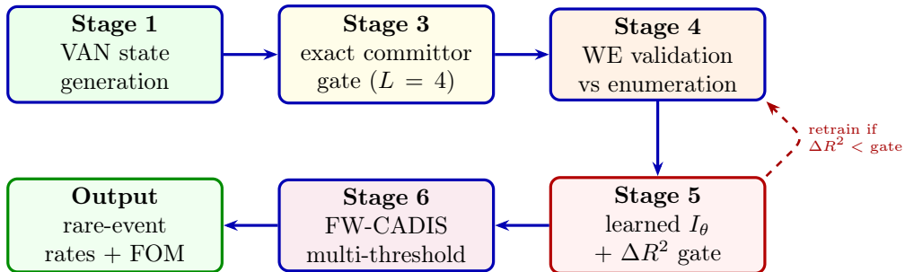
Figure 15: [SCHEMATIC] Execution graph. Every stage is gated against an exact or enumerable reference before the next is trusted; the dashed edge is the diagnostic feedback loop.
