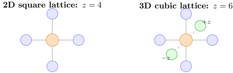
Figure 5: [SCHEMATIC] Nearest-neighbour coordination: a 2D square lattice (left) gives each spin z = 4 neighbours (blue); a 3D cubic lattice (right) adds a third axis (green, dashed bonds shown foreshortened for depth), giving z = 6 . The Hamiltonian’s form, H(s) = -\sum_{\langle i,j \rangle} J_{ij} s_i s_j , is unchanged — only the bond count per site (orange, centre) grows.
