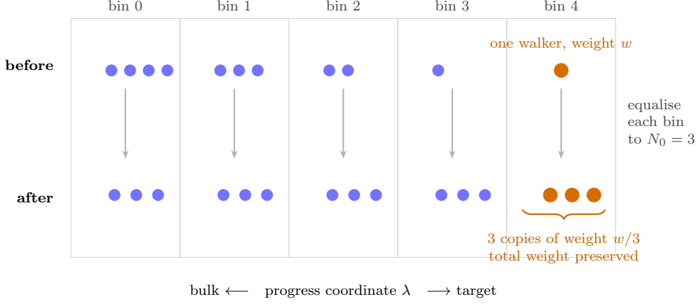
Figure 9: [SCHEMATIC] The whole method in one picture. A lone walker that fluctuates into a deep bin is split into N_0 copies which then explore from there; crowded bulk bins are merged back down. Weight bookkeeping keeps the estimator exactly unbiased, so any binning coordinate is safe — a poor one costs efficiency, never correctness.
