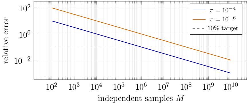
Figure 2: [SCHEMATIC] Exact Poisson relation (9), not fitted data. Each decade of rarity costs a decade of samples. This is the wall the project exists to get around.
