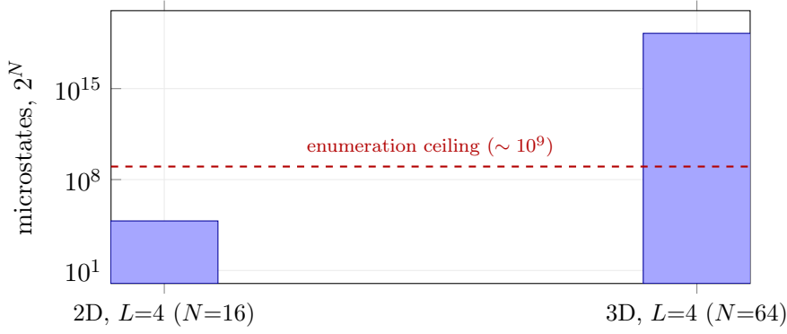
Figure 6: [SCHEMATIC] Exact-enumeration cost at L = 4 : trivial in 2D ( 2^{16} = 65536 states), utterly infeasible in 3D ( 2^{64} \approx 1.8 \times 10^{19} states) — fourteen orders of magnitude beyond any practical enumeration budget. This is why the L = 4 validation strategy used throughout this manual (§5.2) cannot simply be re-run one dimension higher.
