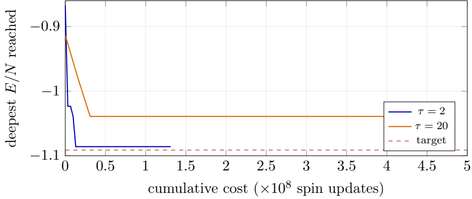
Figure 11: [MEASURED] Identical bins, one seed. At \tau = 2 the front reaches -1.086 by cost 1.3 \times 10^8 and plateaus because it has arrived . At \tau = 20 it plateaus at -1.039 because it is stuck , then spends 3.7\times more budget going nowhere. Both plateaus look alike; only one is convergence.
