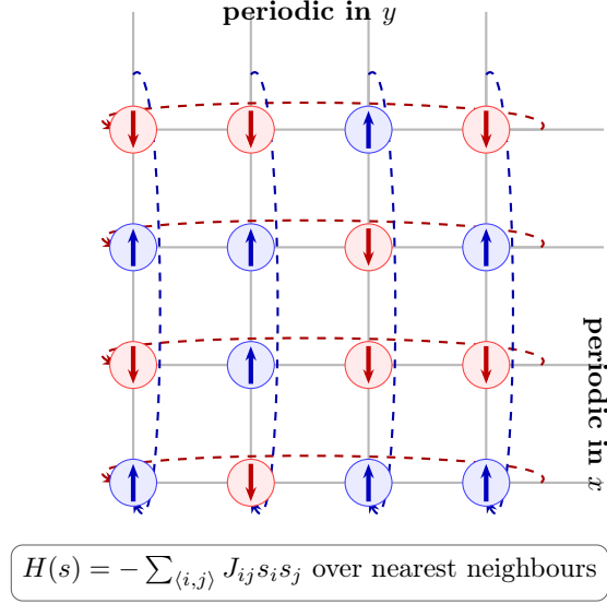
Figure 3: [SCHEMATIC] The L \times L lattice, drawn at L = 4 . Blue = spin up, red = spin down, solid lines are coupling bonds J_{ij} , dashed arrows are the periodic identifications.
