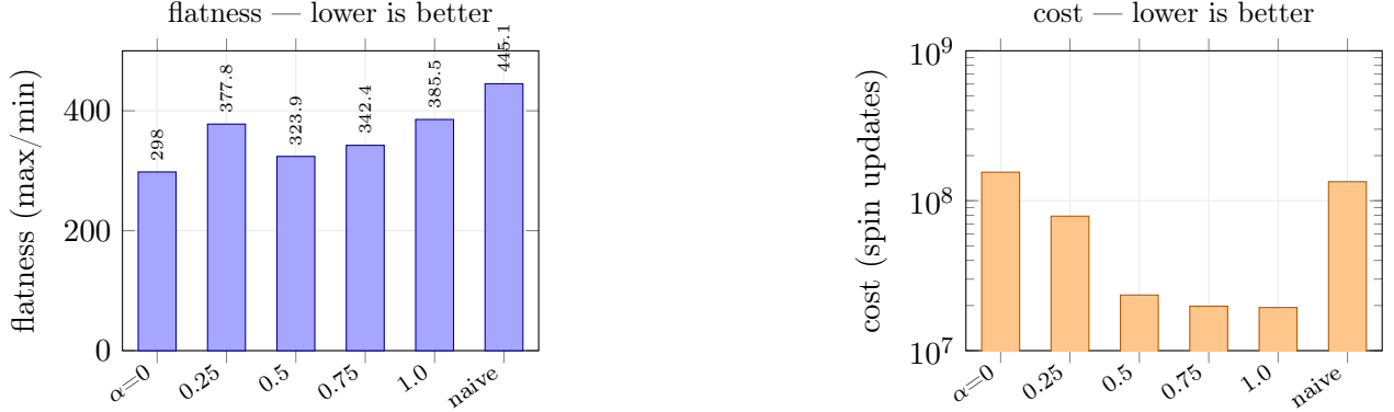
Figure 14: [MEASURED] EA spin glass, L = 16 , R = 30 , 6 thresholds, full 6/6 coverage at every allocation. Left: uniform allocation ( \alpha = 0 ) is the flattest ; every FW-CADIS setting is worse, and not even monotonic in \alpha . Right: FW-CADIS runs at \sim 8\times lower cost. The cost advantage is real; the flattening advantage is not present.
