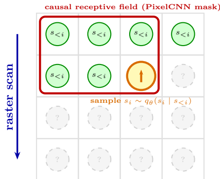
Figure 12: [SCHEMATIC] Autoregressive generation. Type-A masking (first layer) zeroes the centre pixel to prevent self-dependence; type-B masking (later layers) retains it.
