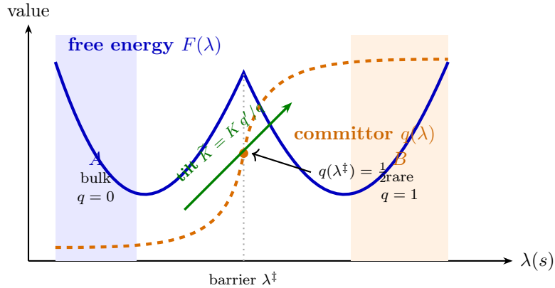
Figure 8: [SCHEMATIC] The committor is smooth and monotone where the free energy has a barrier. Tilting by q converts the barrier into a downhill drift, which is why the estimator becomes variance-free. Curves are illustrative shapes, not measured profiles.
