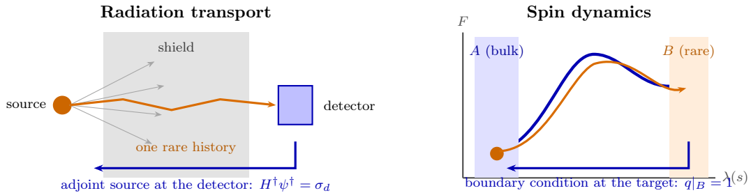
Figure 7: [SCHEMATIC] The same structure twice. Both quantities are defined backward from the target : the adjoint source sits at the detector, the committor boundary condition sits on the rare set. That shared direction is the whole correspondence, and it is why transport’s variance-reduction toolkit transfers.
