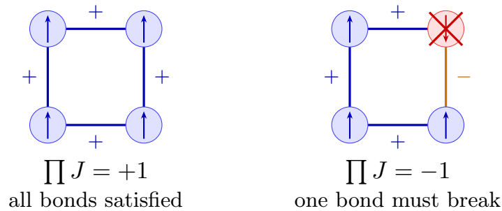
Figure 4: [SCHEMATIC] Left: all four bonds ferromagnetic, product +1 , a satisfying assignment exists. Right: one antiferromagnetic bond makes the product -1 ; whichever spins are chosen, at least one bond is unsatisfied. Frustration is what makes the energy landscape rugged.
