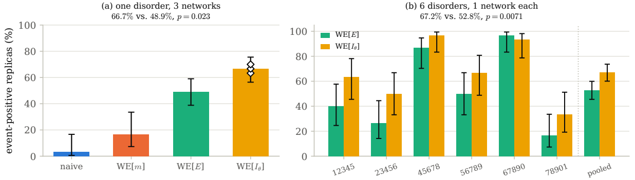
Figure 2: The learned importance coordinate reaches the deep target more reliably than the physical energy coordinate. Error bars are Wilson 95% intervals. (a) Discovery rate at beyond = 4 (disorder realization 12345): open diamonds are the three independently trained networks (Table 4); WE[E] uses the balanced 90-replica baseline. (b) The same comparison repeated across six independent disorder realizations, one trained network each (Table 5), with the pooled result at right.
