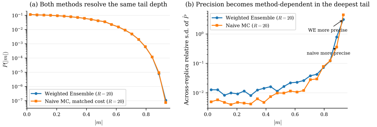
Figure 1: L = 20 Ising magnetization tail at matched spin-update cost, R = 20 independent replicas per method. (a) P(|m|) on a log scale: the WE and naive curves are visually indistinguishable through the bulk and near tail, and both resolve the tail to the identical deepest bin, |m| = 0.932 . (b) Across-replica relative standard deviation of \hat{P}(|m|) on a log scale: naive sampling holds the lower (better) relative s.d. through most of the tail, and only WE becomes more precise at the single deepest bin, annotated directly on the plot.
