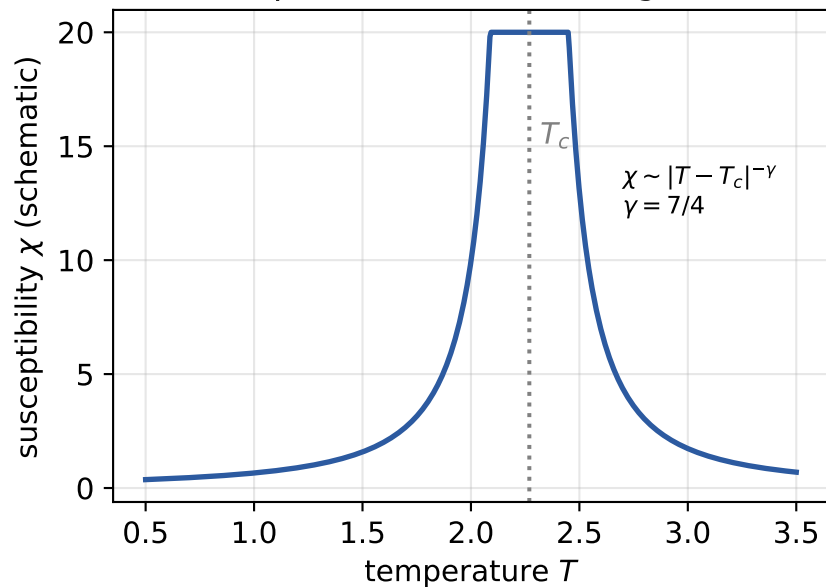
(b) Response function diverges at T_c
