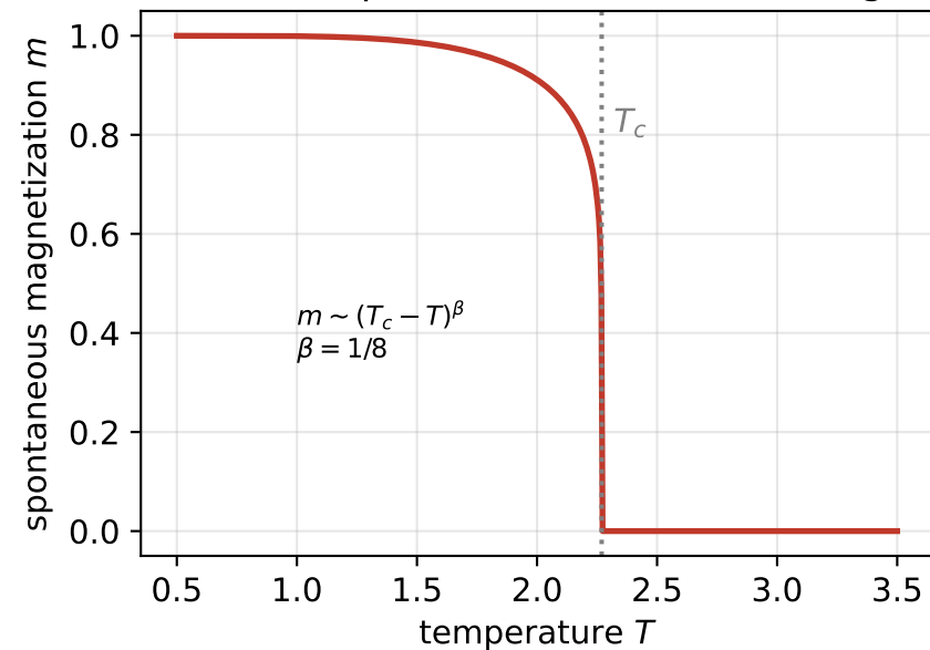
(a) Order parameter (exact, 2D Ising)
