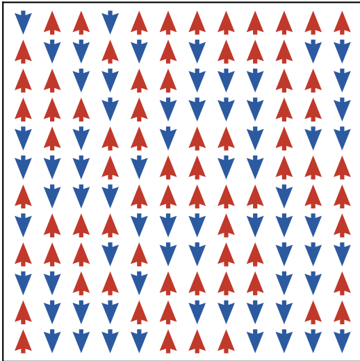
Paramagnet (disordered, fluctuating)
