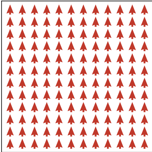
Ferromagnet m \neq 0 , uniform
