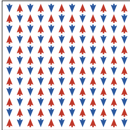
Antiferromagnet staggered m_s \neq 0
