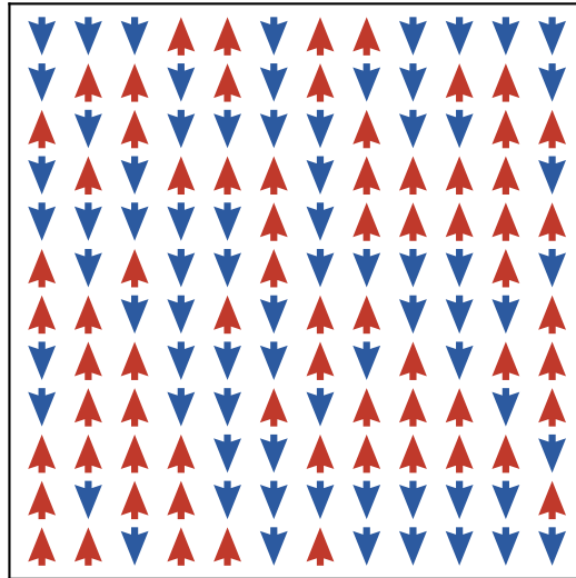
Spin glass (frozen, random)
