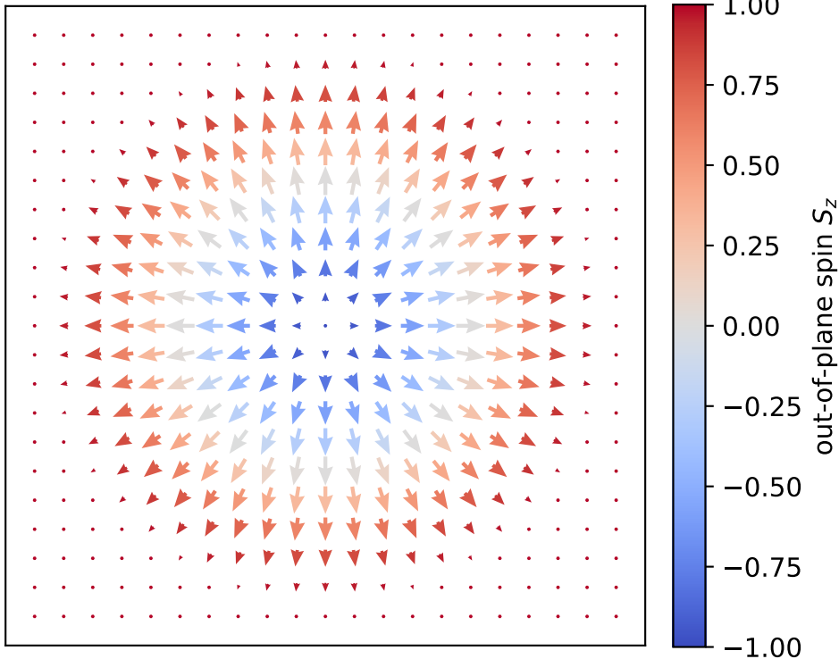
Magnetic skyrmion (topological winding number Q = 1 )
